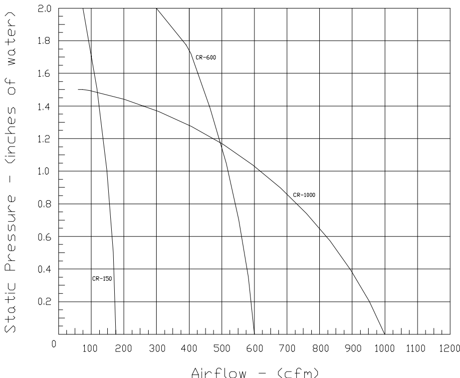
Fan Performance Curves
